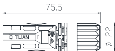
Conector macho (-)
